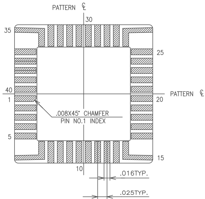
BONDING PATTERN
