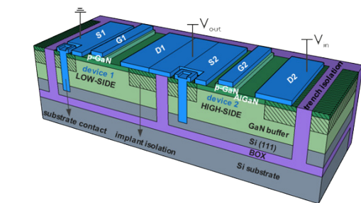
Schematic cross-section of monolithically integrated half-bridge with enhancement mode low-side and high-side devices fabricated on 200 nm GaN-on-SOI with trench isolation.
