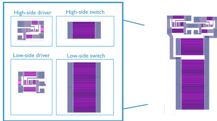
Monolithic integration of half-bridge and gate driver on imec's GaN IC platform.
