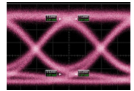
50Gb/s, 2.5Vpp
